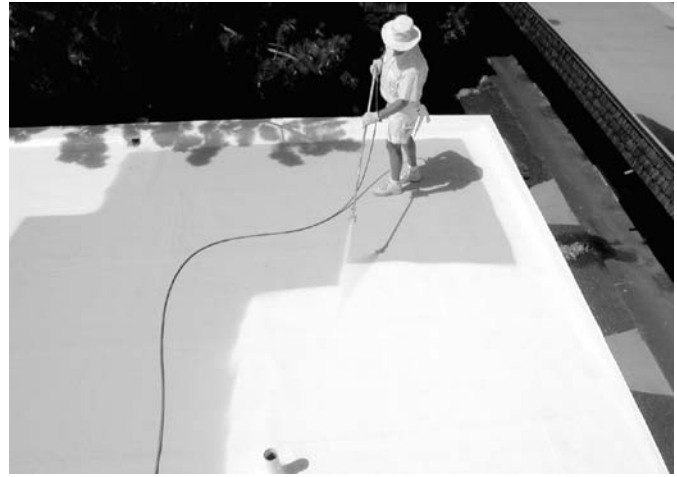
White coatings can be applied on many roof types, including this old BUR on an apartment building. The white coating is sprayed over a base coat on top of an old built-up roof.
