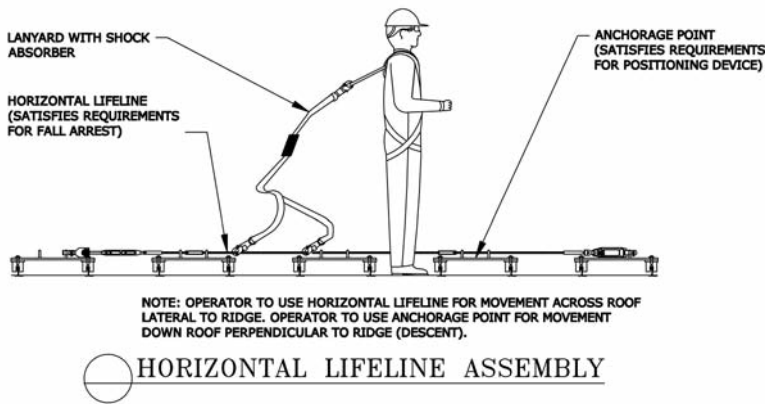
Figure 1 – CAD image of noninvasive anchorage points and horizontal lifeline assembly. System is designed for fall-arrest and position-device requirements.
